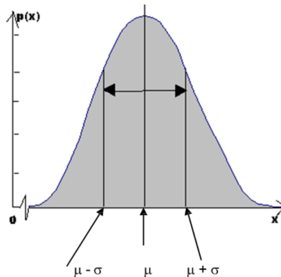
Fig 1: Normal or Gaussian distribution
