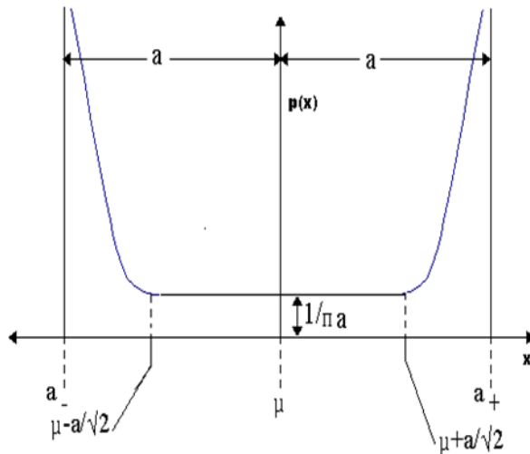
Fig 4 : Schematic of U-shaped distribution
