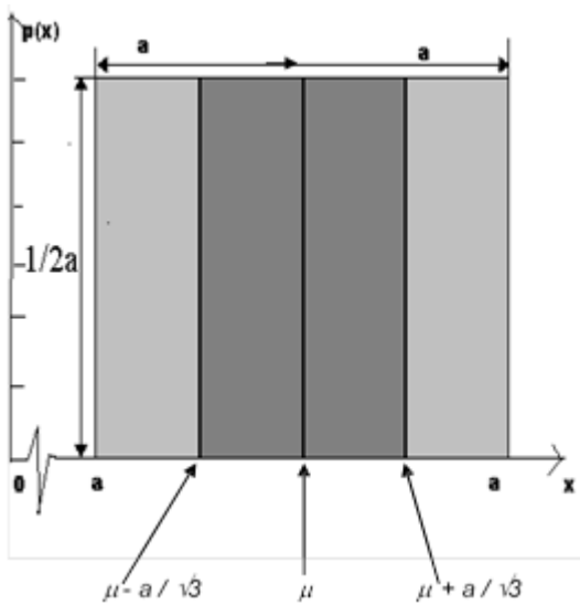
Fig 2 : Schematic of the rectangular distribution
